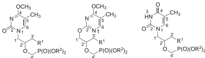
FIG. 1 General numbering scheme for assignment of NMR signals
